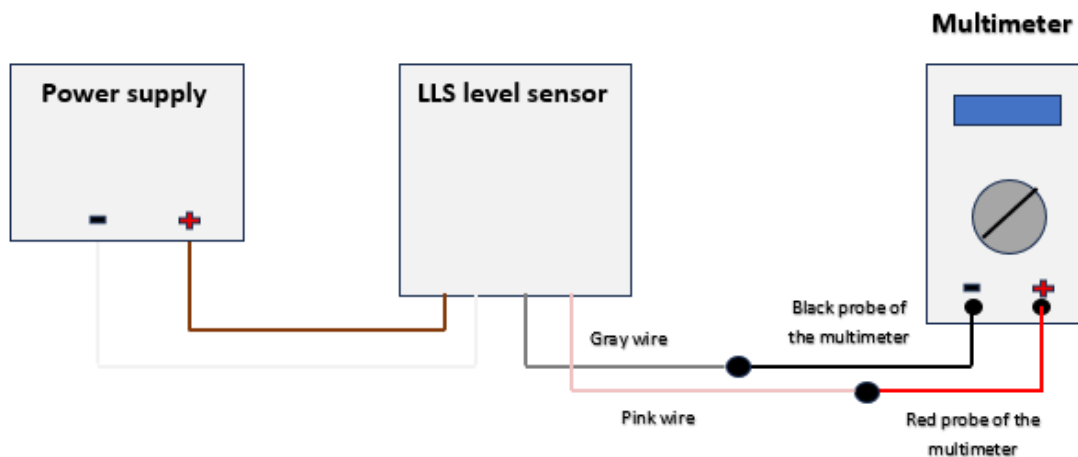
Fig. 8 Connection Diagram
