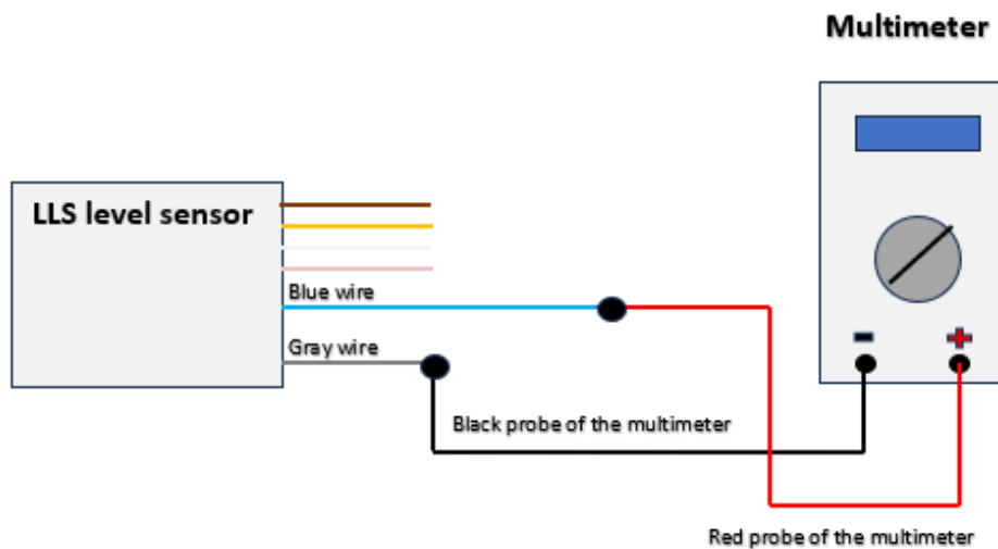
Fig. 11 Connection Diagram
